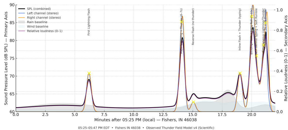
Observed Thunder Field — Stereo Thunder Roll (Left → Right), Lightning & Rain
